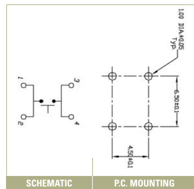
SCHEMATIC
