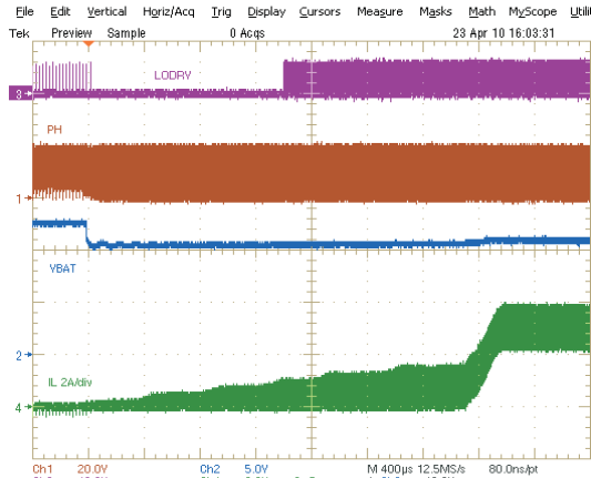
CH1: PHASE, 20V/div, CH2: battery voltage, 5V/div, CH3: L0DRV, 10V/div, CH4: inductor current, 2A/div, 400us/div
