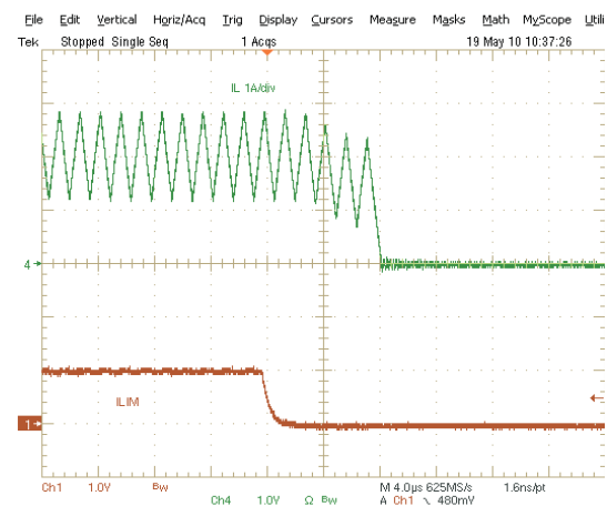
Figure 6. Charge Enable by ILIM
