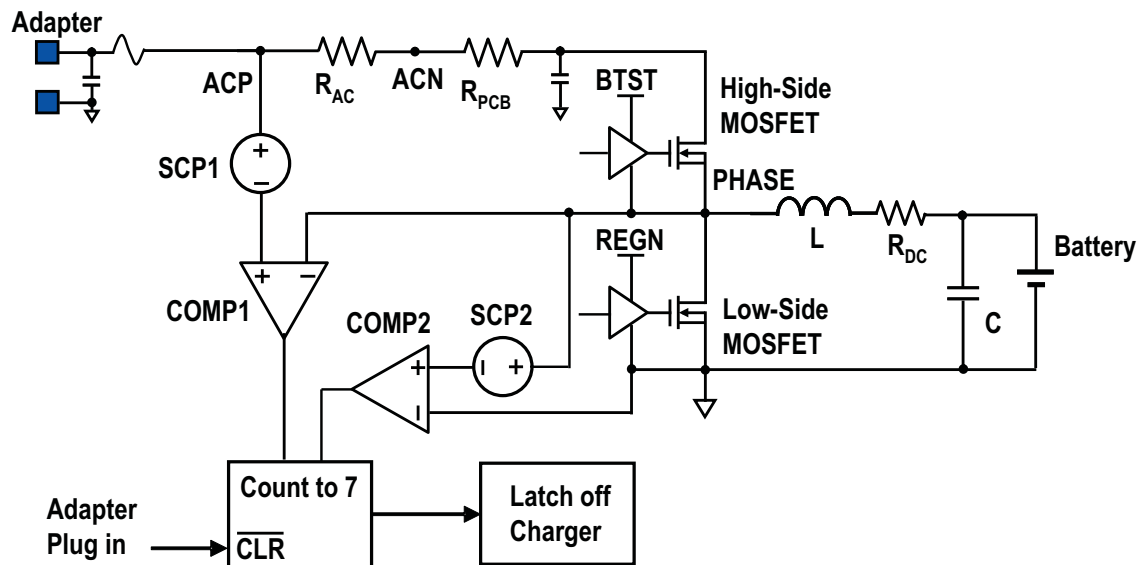
Figure 20. Block Diagram of bq24725A Short Circuit Protection
