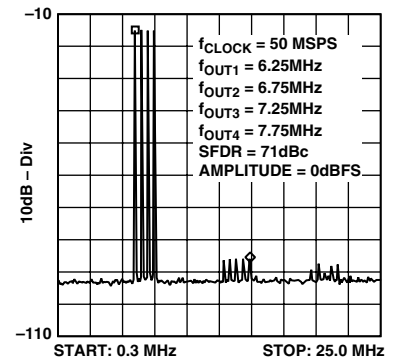
Figure 38. Four-Tone SFDR
