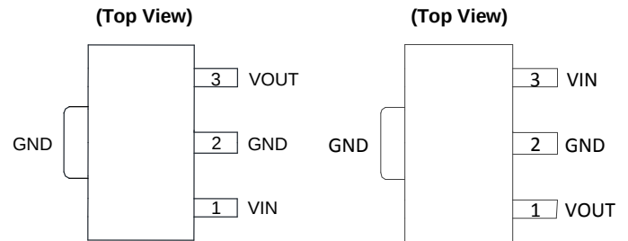
SOT89 (Note 1)
