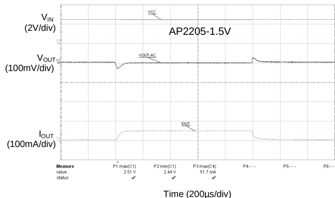
Load Transient (Conditions: V_{IN}=2.5V , C_{IN}=1.0\mu F , C_{OUT}=2.2\mu F , I_{OUT}=1mA to 50mA )
