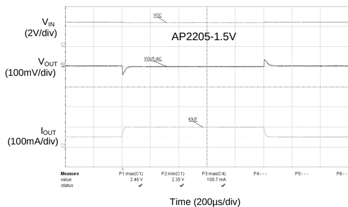
Load Transient (Conditions: V_{IN}=2.5V , C_{IN}=1.0\mu F , C_{OUT}=2.2\mu F , I_{OUT}=50mA to 100mA )
