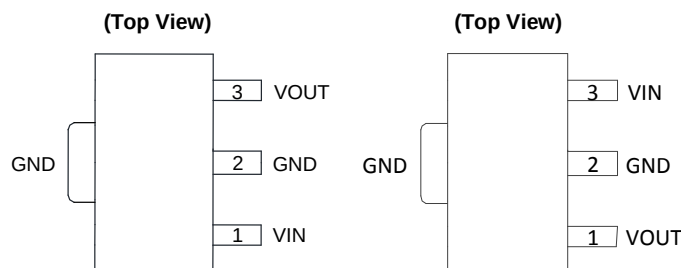
SOT89 (Note 1)
