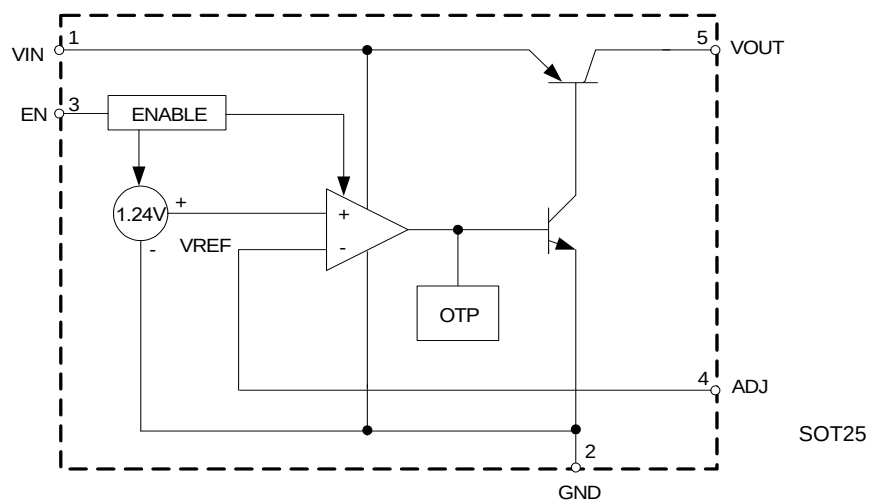
Adjustable Version
