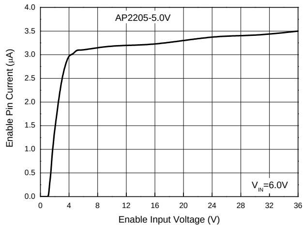
Enable Pin Current vs. Enable Input Voltage
