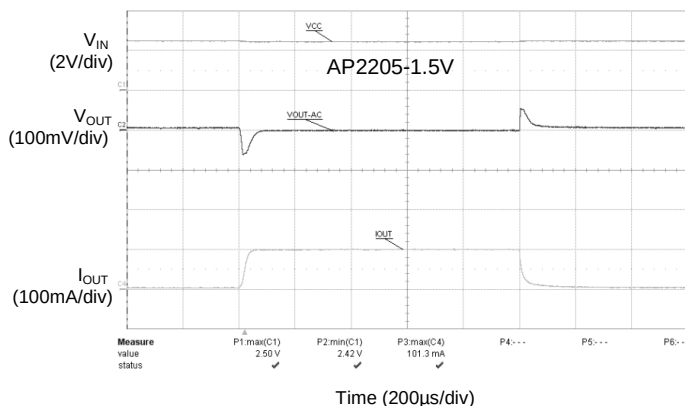
Load Transient (Conditions: V_{IN}=2.5V , C_{IN}=1.0\mu F , C_{OUT}=2.2\mu F , I_{OUT}=1mA to 100mA )
