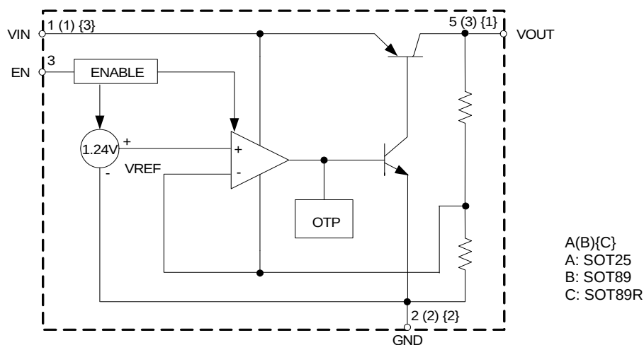
Fixed Version
