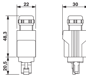
Push-pull RJ45 connector IP65/67
