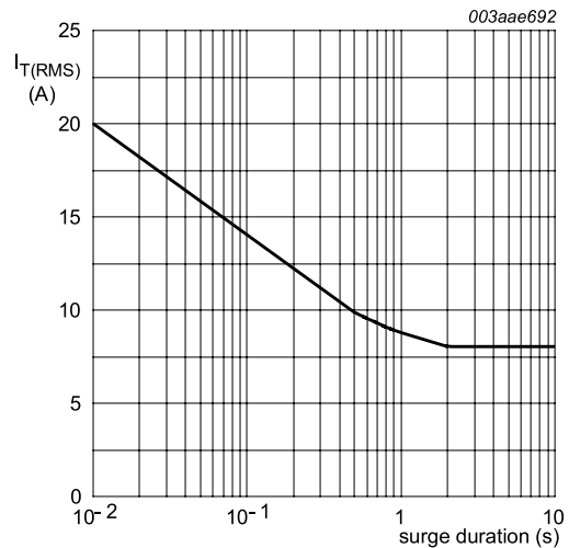
Fig. 2. RMS on-state current as a function of surge duration; maximum values f = 50 Hz; T_{mb} \leq 102^\circ\text{C}
