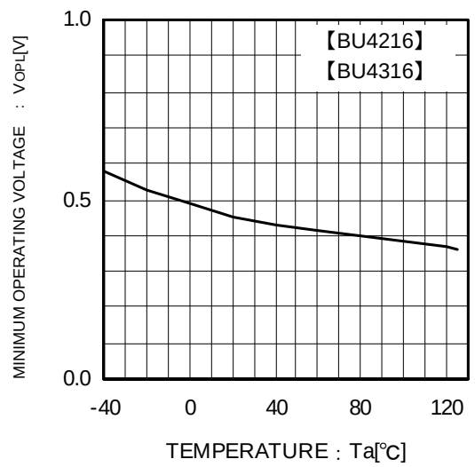
Fig.12 Operating Limit Voltage
