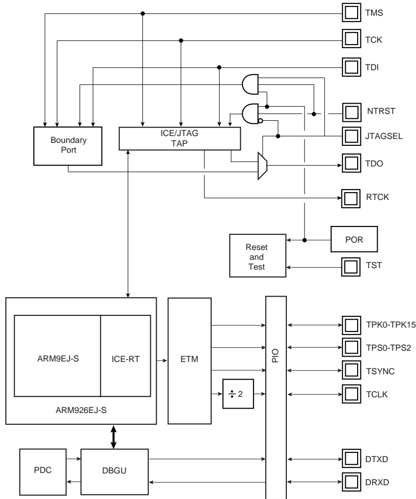
Figure 11-1. Debug and Test Block Diagram
