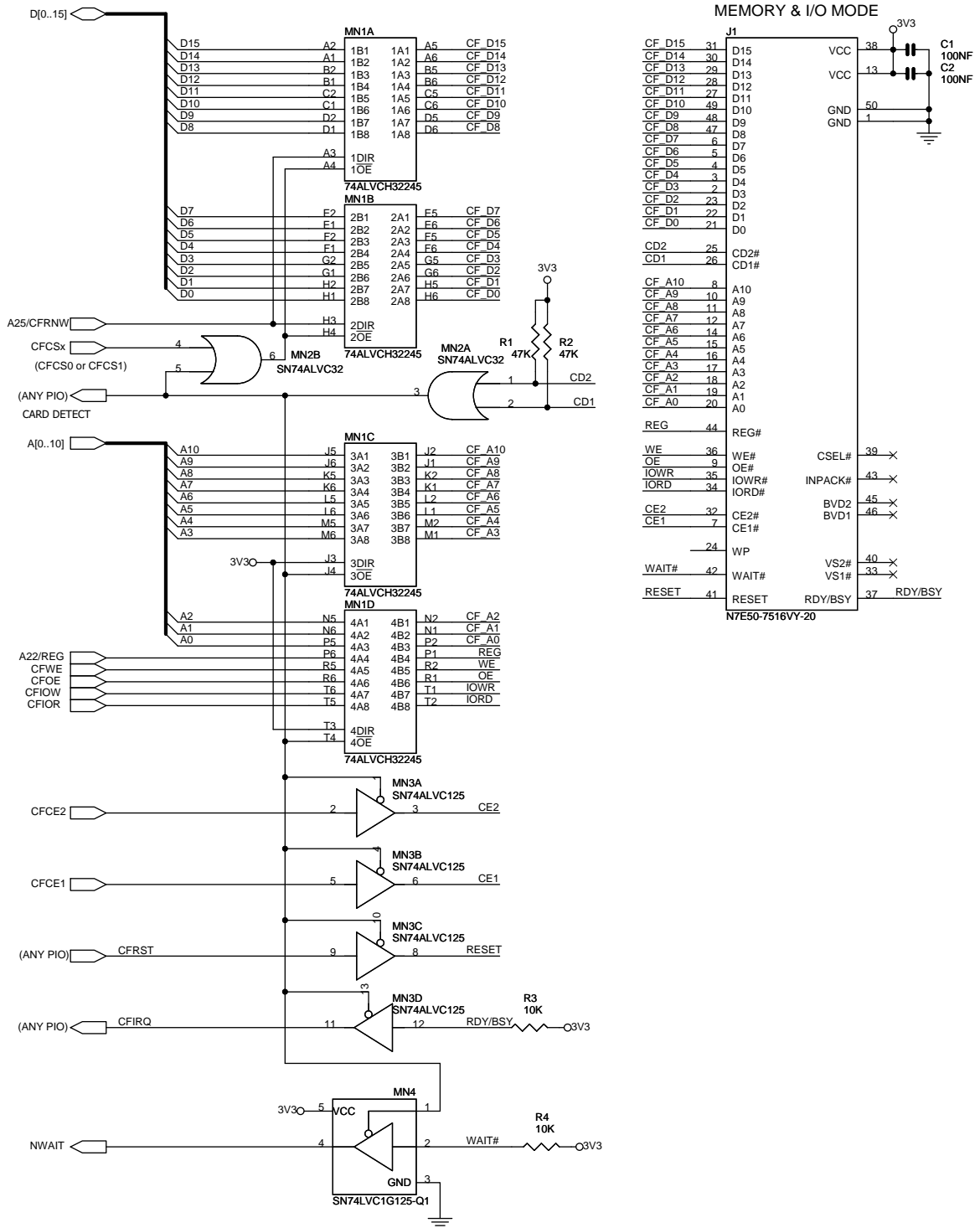
Figure 19-8. Hardware Configuration
