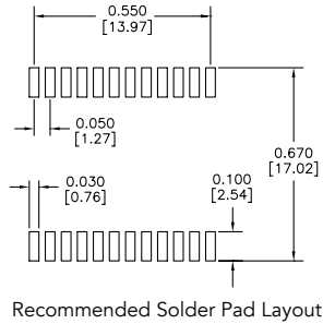
Recommended Solder Pad Layout
