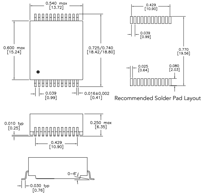
Dimensions: inch [mm]
