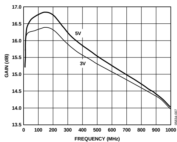
Figure 7. Gain vs. Frequency and Supply, V_{POS} = 5\text{ V} and 3\text{ V}
