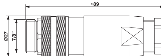
Dimensioned drawing
