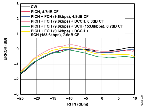
Figure 27. Error from CW Linear Reference vs. Input with Various CDMA2000 Reverse Link Waveforms at 900 MHz, C_{FILTR} = 1 nF, C_{OUT} = 100 nF
