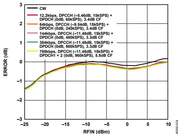
Figure 24. Error from CW Linear Reference vs. Input with Various WCDMA Up Link Waveforms at 1900 MHz, C_{FILTR} = Open, C_{OUT} = 100 nF
