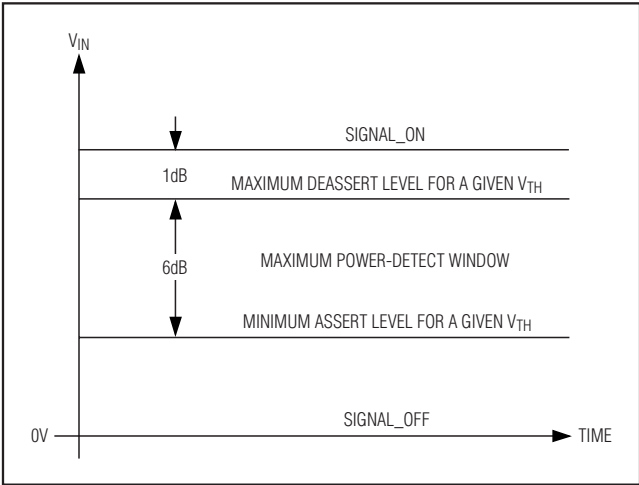
Figure 2A. LOS Deassert Threshold—Set 1dB Below Receiver Sensitivity
