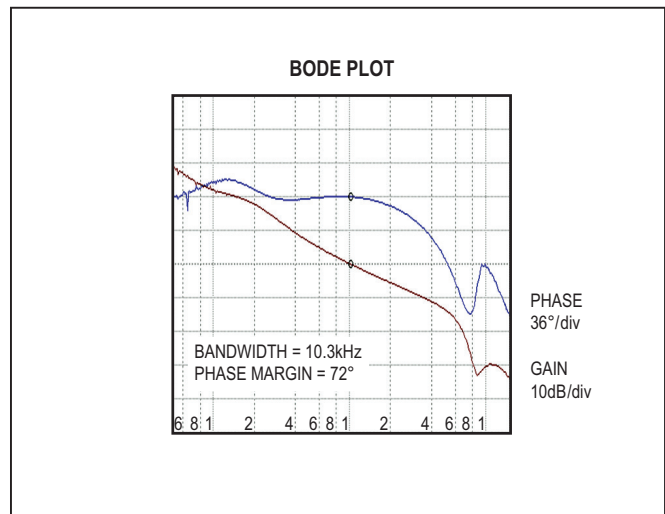
Figure 4. Bode Plot
