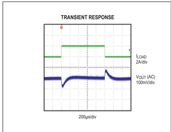
Figure 3. Transient Response
