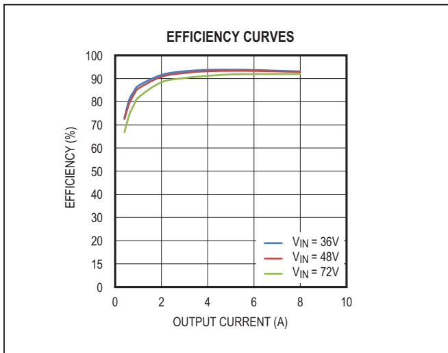
Figure 1. Efficiency Curves
