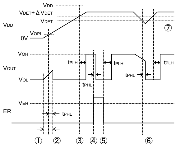
Fig.17 Timing Waveform
