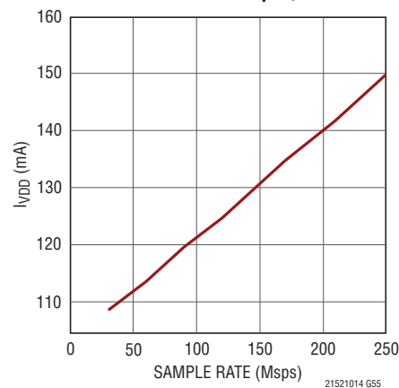
LTC2150-14: I_{VDD} vs Sample Rate, 15\text{MHz} Sine Wave Input, -1\text{dBFS}
