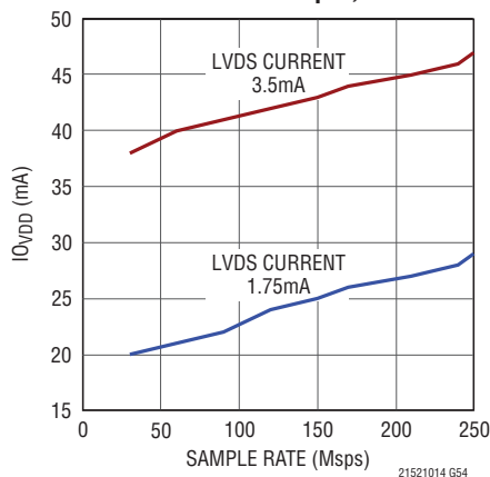
LTC2150-14: I_{OVD} vs Sample Rate, 15\text{MHz} Sine Wave Input, -1\text{dBFS}
