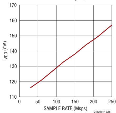
LTC2151-14: I_{VDD} vs Sample Rate, 15MHz Sine Wave Input, -1\text{dBFS}
