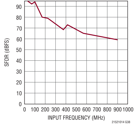
LTC2151-14: SFDR vs Input Frequency, -1dBFS, 1.5V Range, 210Mps
