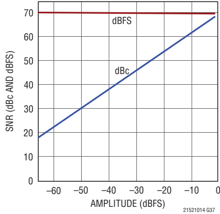
LTC2151-14: SNR vs Input Level, f_{IN} = 71\text{MHz} , 1.5V Range, 210Mps
