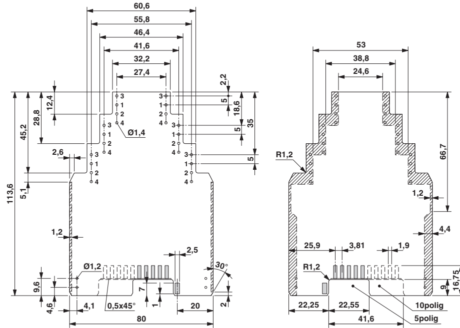
Dimensioned drawing
