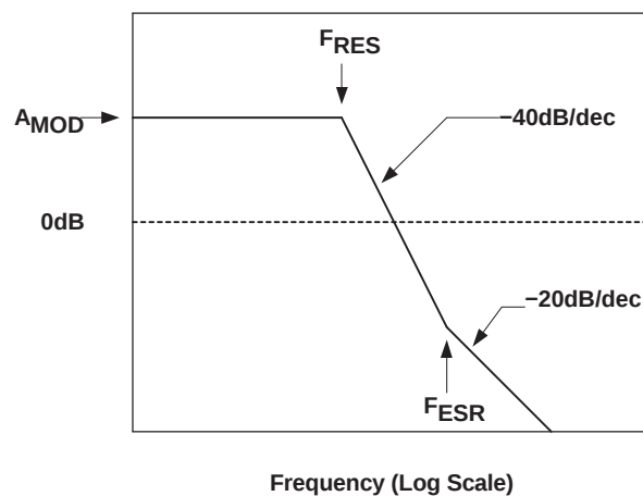
Figure 20. Power Stage Frequency Response Straight Line Approximation
