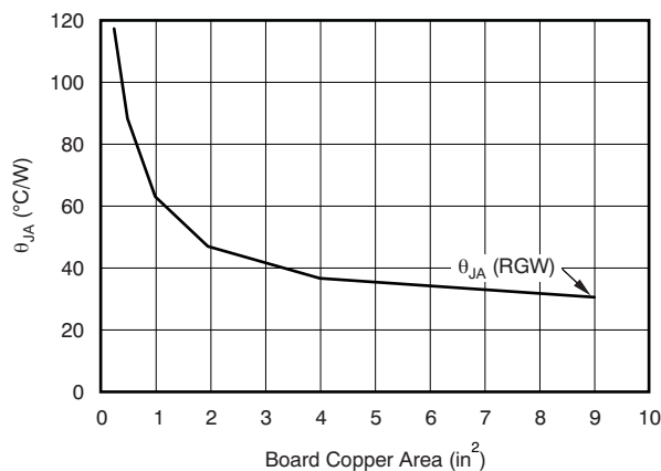
Figure 25. \theta_{JA} vs Board Size
