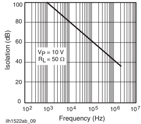
Fig. 10 - Output Isolation
