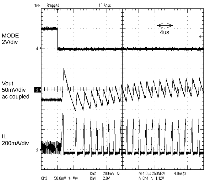
Figure 46. Mode Change Response MODE : High to Low
