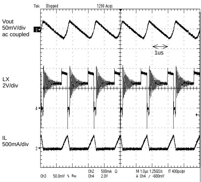
Figure 44. PFM mode Operation Iout=50mA
