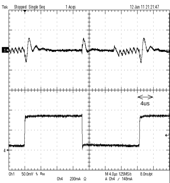
Figure 31. Load transient response 50mA to 350mA t_r=t_f=100\text{ns} , Mode :Low
