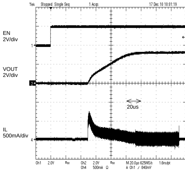
Figure 5. Start up
