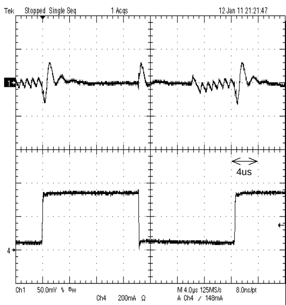
Figure 31. Load transient response 50mA to 350mA tr=tf=100ns, Mode :Low
