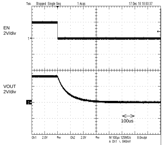
Figure 6. Shut down
