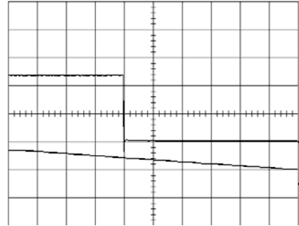
Shut-down enabled by disconnecting V_i at: T_{ref} = +25^\circ\text{C} , I_O = 10\text{ A} resistive load, V_i = 12.0\text{ V} . Top trace: output voltage (0.5 V/div.). Bottom trace: input voltage (10 V/div.). Time scale: 5.0 ms/div.
