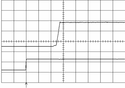
Start-up enabled by connecting V_i at: T_{ref} = +25^\circ\text{C} , I_O = 10\text{ A} resistive load, V_i = 12.0\text{ V} . Top trace: output voltage (0.5 V/div.). Bottom trace: input voltage (10 V/div.). Time scale: 5 ms/div.
