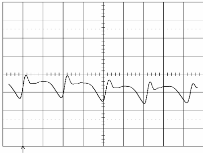
Output voltage ripple (20mV/div.) at: T_{ref} = +25^\circ\text{C} , I_O = 10\text{ A} resistive load, V_i = 12.0\text{ V} . Time scale: 2 \mu\text{s} /div. See the filter in the Output ripple and noise section (EMC Specification).
