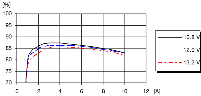
Efficiency vs. load current and input voltage at T_{ref} = +25^{\circ}C
