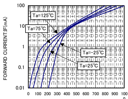
FORWARD VOLTAGE:VF(mV) VF-IF CHARACTERISTICS VF分布
