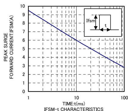
IFSM-t CHARACTERISTICS
