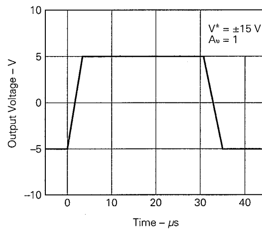
PULSE RESPONSE
