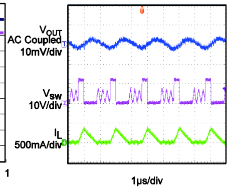
Output Voltage Ripple I_{OUT}=0.1A
