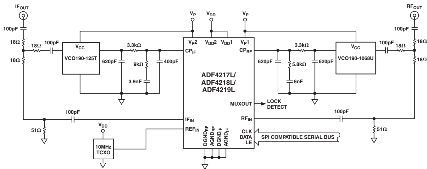
Figure 7. Local Oscillator Design for GSM Receiver
