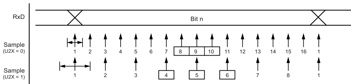
Figure 17-6. Sampling of Data and Parity Bit
