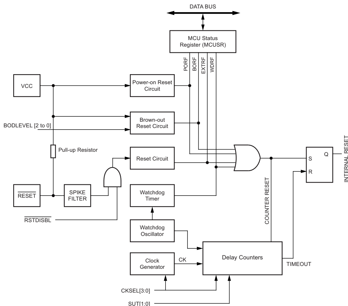
Figure 8-1. Reset Logic
