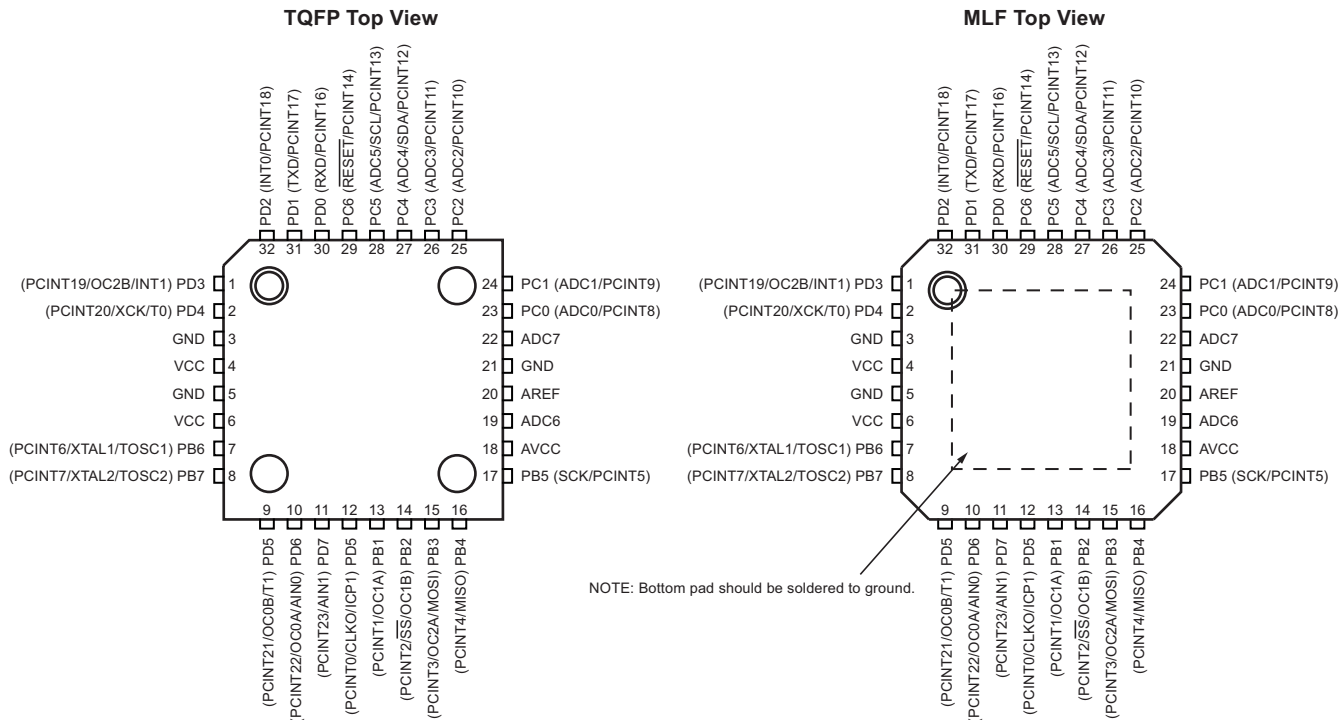
Figure 1-1. Pinout ATmega48/88/168
