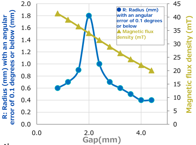
CM9BI Measured value using a dual-form magnet with a \Phi 13 x thickness
