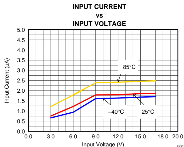
Figure 22. Shutdown Current
