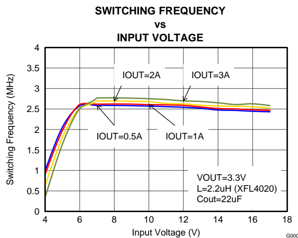
Figure 19. Switching Frequency
