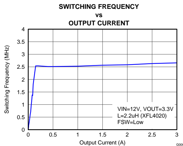
Figure 20. Switching Frequency
