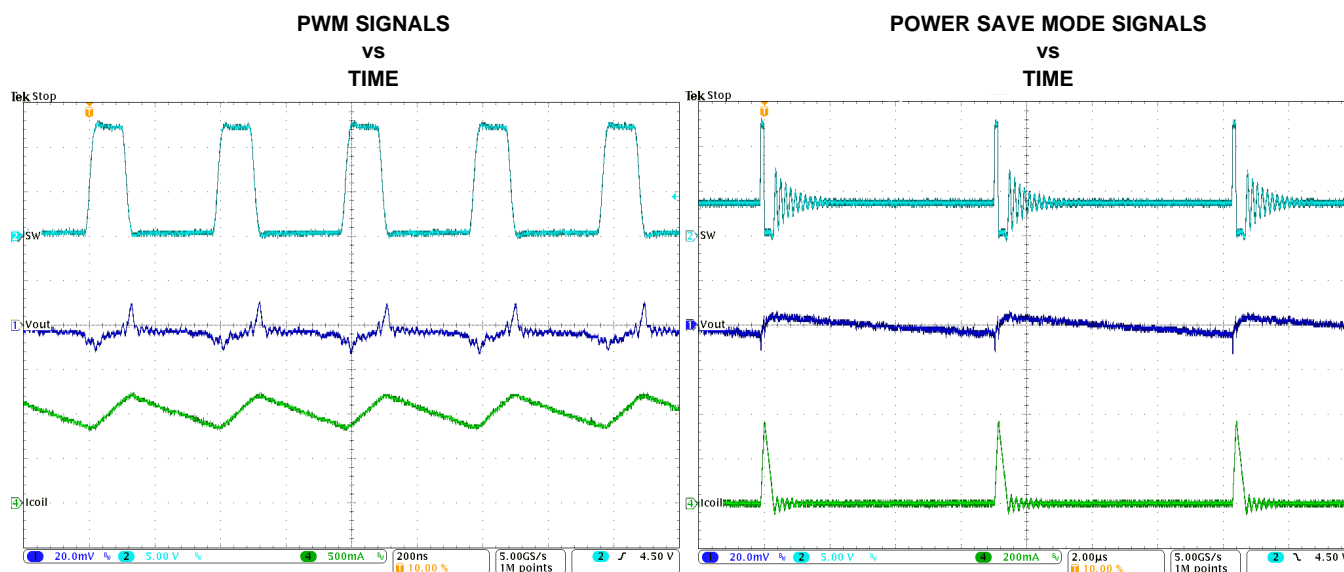
Figure 35. Typical Operation in PWM Mode (IOUT=1A)
