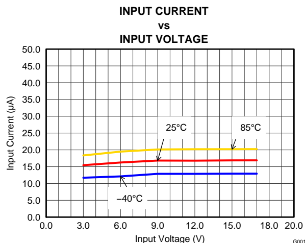
Figure 21. Quiescent Current
