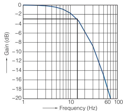
5. Frequency characteristics
