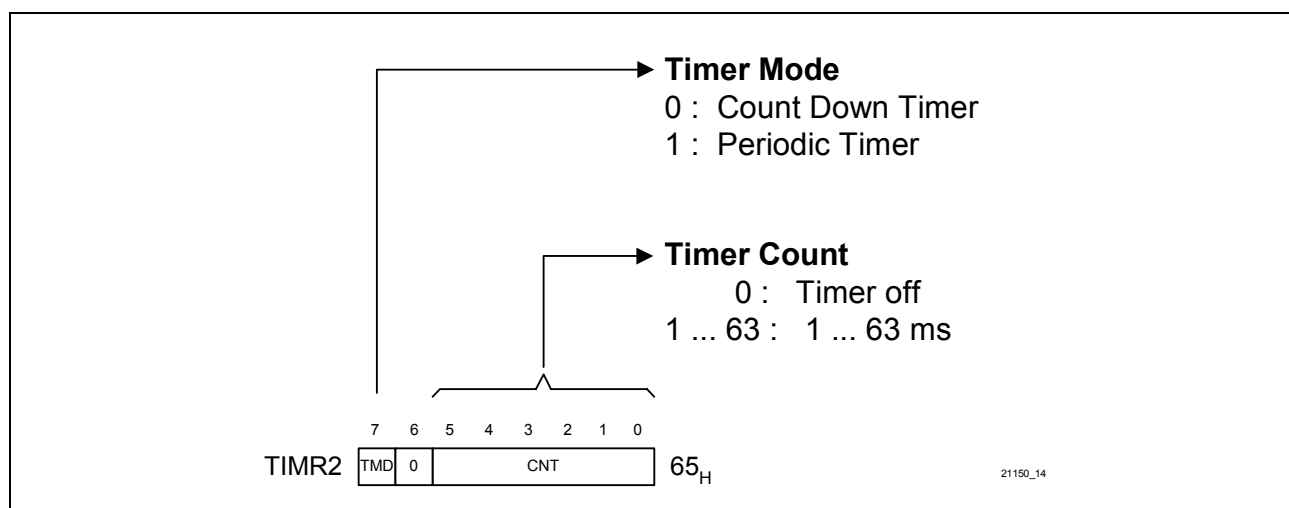
Figure 12 Timer 2 Register
