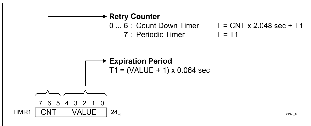
Figure 11 Timer 1 Register
