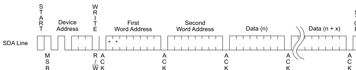
Figure 8-2. Page Write
