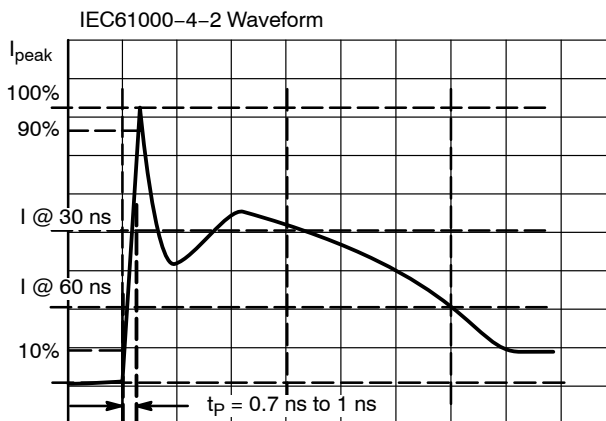
Figure 9. IEC61000-4-2 Spec
