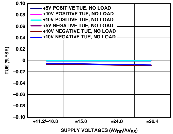
Figure 14. Total Unadjusted Error vs. Supply Voltages
