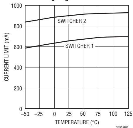
Switching Regulator Current Limit
