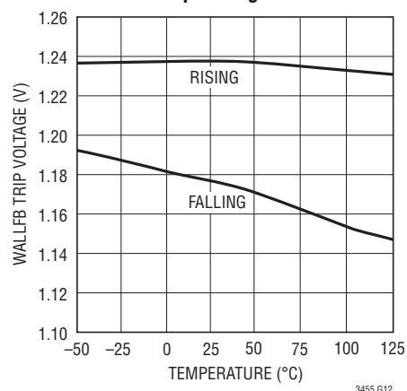
WALLFB Trip Voltage
