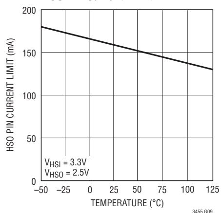
HSO Pin Current Limit
