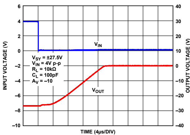
Figure 57. Negative Overload Recovery, V_{SY} = \pm 27.5V
