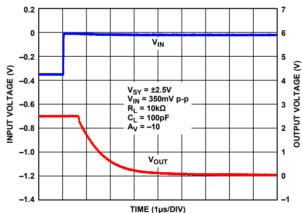
Figure 52. Positive Overload Recovery, V_{SY} = \pm 2.5V
