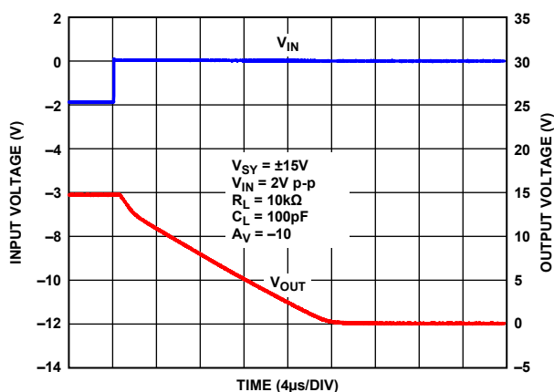
Figure 53. Positive Overload Recovery, V_{SY} = \pm 15V
