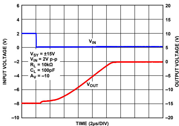
Figure 56. Negative Overload Recovery, V_{SY} = \pm 15V
