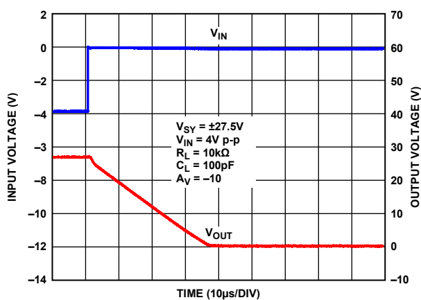
Figure 54. Positive Overload Recovery, V_{SY} = \pm 27.5V
