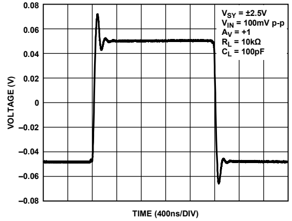
Figure 37. Small Signal Transient Response, V_{SY} = \pm 2.5 V
