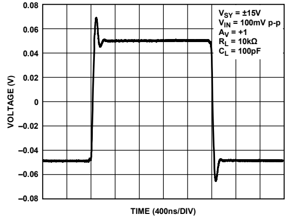
Figure 38. Small Signal Transient Response, V_{SY} = \pm 15 V
