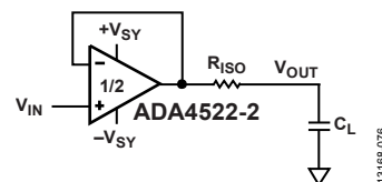
Figure 77. Stability Compensation with Isolating Resistor, R_{ISO}
