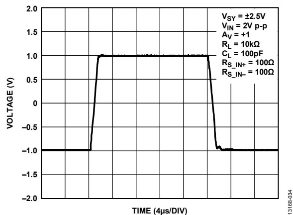
Figure 34. Large Signal Transient Response, V_{SY} = \pm 2.5\text{ V}
