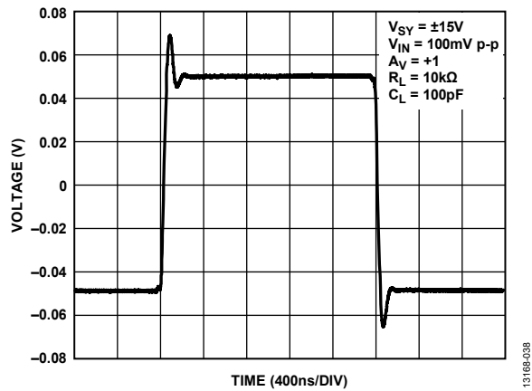
Figure 38. Small Signal Transient Response, V_{SY} = \pm 15\text{ V}
