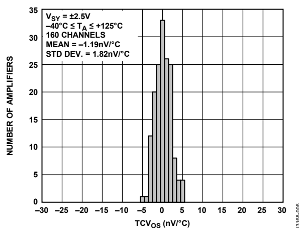
Figure 7. Input Offset Voltage Drift Distribution, V_{SY} = \pm 2.5\text{ V}
