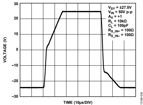
Figure 36. Large Signal Transient Response, V_{SY} = \pm 27.5\text{ V}
