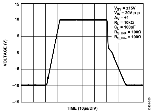
Figure 35. Large Signal Transient Response, V_{SY} = \pm 15\text{ V}
