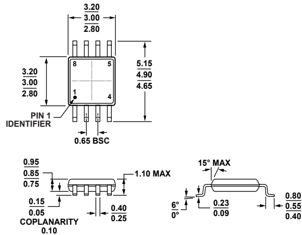
COMPLIANT TO JEDEC STANDARDS MO-187-AA Figure 86. 8-Lead Mini Small Outline Package [MSOP] (RM-8) Dimensions shown in millimeters
