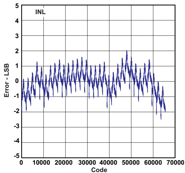
Figure 1. Integral Non-Linearity
