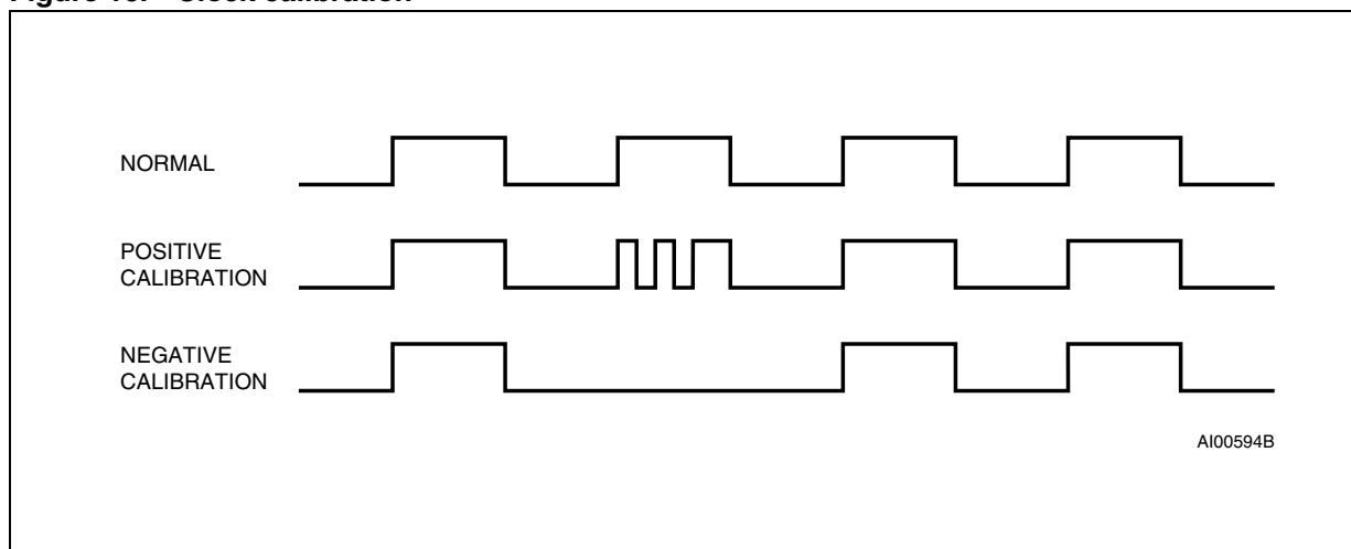
Figure 10. Clock calibration
