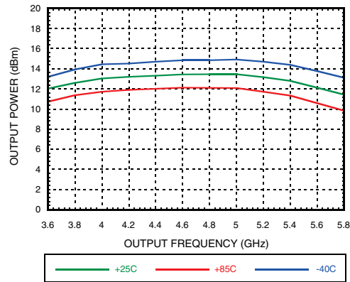
Output Power vs. Temperature @ 0 dBm Drive Level
