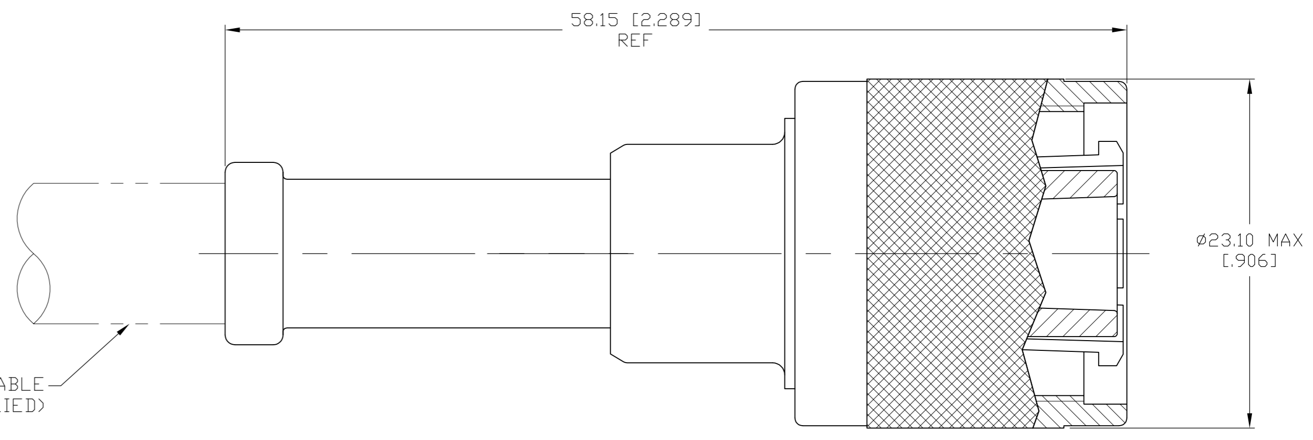
ASSEMBLED VIEW
