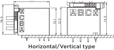
Horizontal/Vertical type
