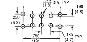
2 Pole P.C. Mounting
