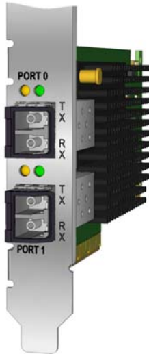
Figure 14 OCe14101B-NM/-NX, OCe14102B-NM/-NX, and OCe14102B-UX/-UM Adapter LED Indicators
