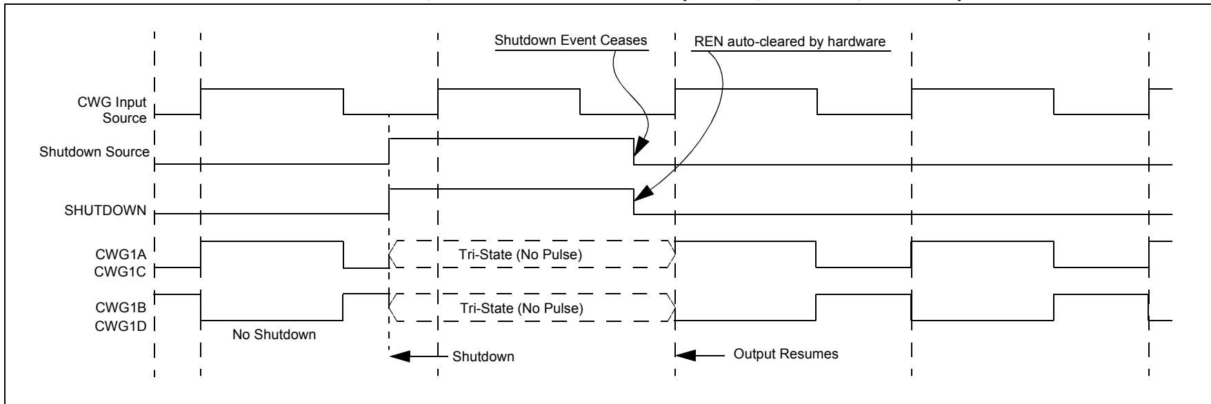
FIGURE 30-14: SHUTDOWN FUNCTIONALITY, AUTO-RESTART ENABLED (REN = 1, LSAC = 01, LSB = 01)
